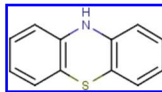
Figure 1. Chemical structure of phenothiazine.
